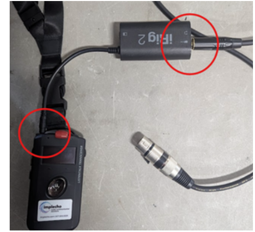
iRIG cable connection through an audio connection on the soundboard
